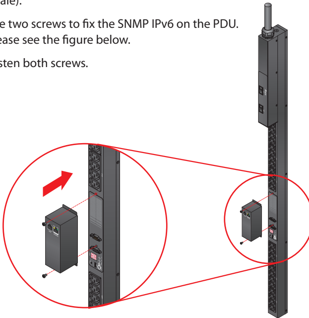
(Figure 3-a : Install the SNMP IPv6 on your PDU)
