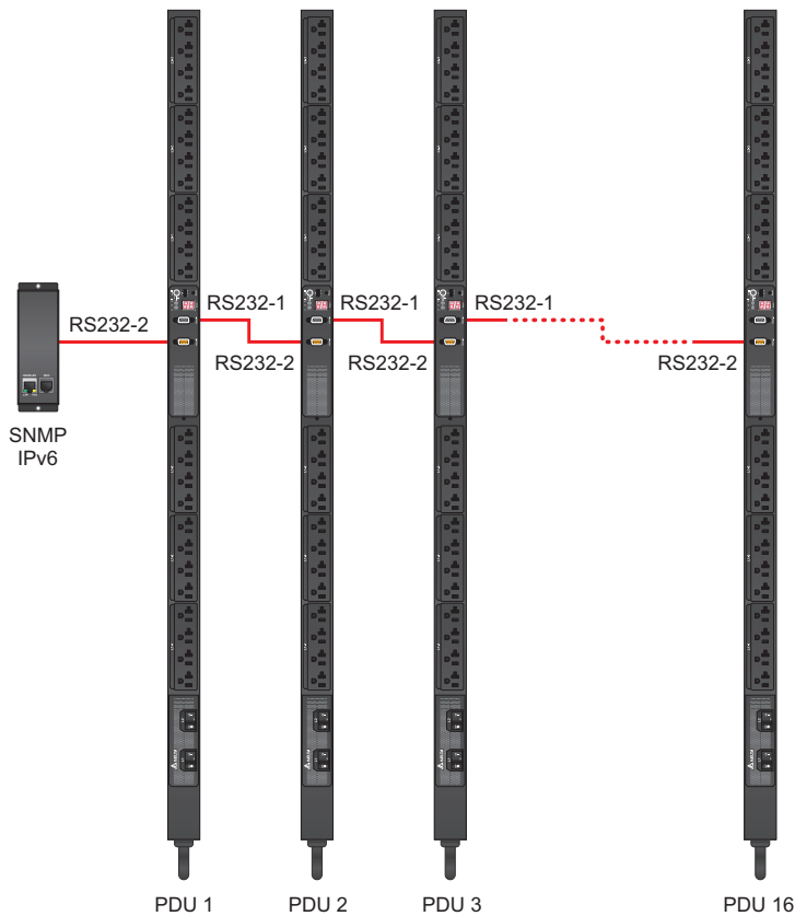
(Figure 3-b : Connection of Multiple PDU Devices)
