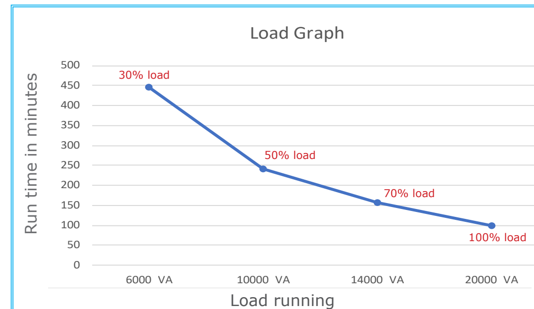
Load Graph
